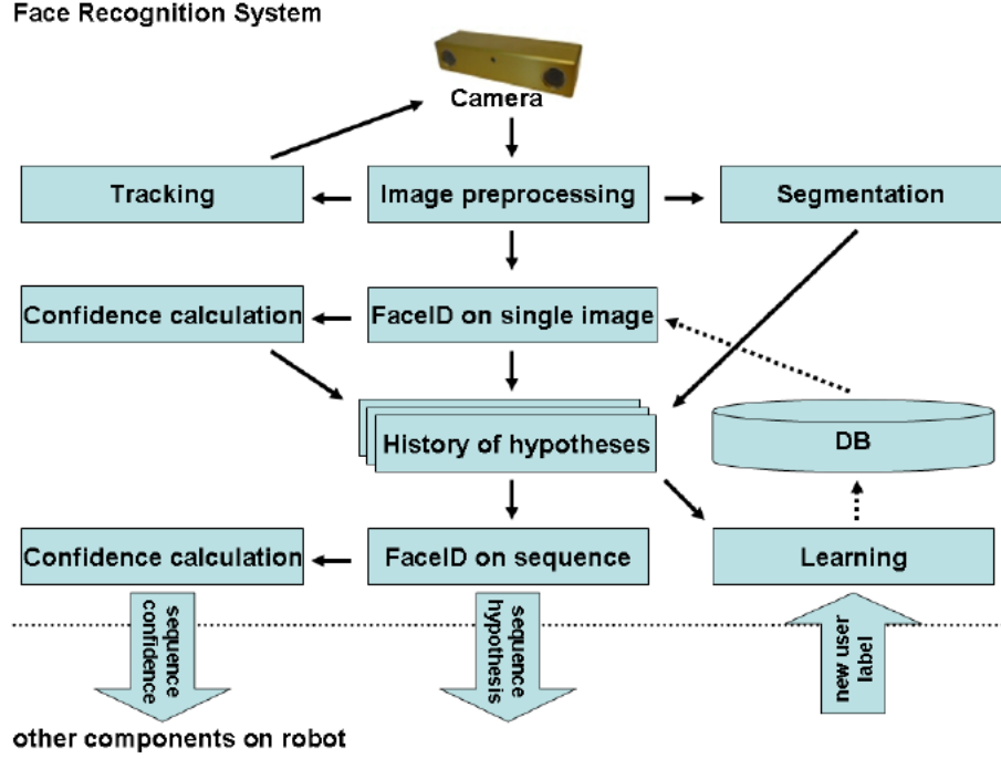
Figure 4.1: System architecture of face recognition system
